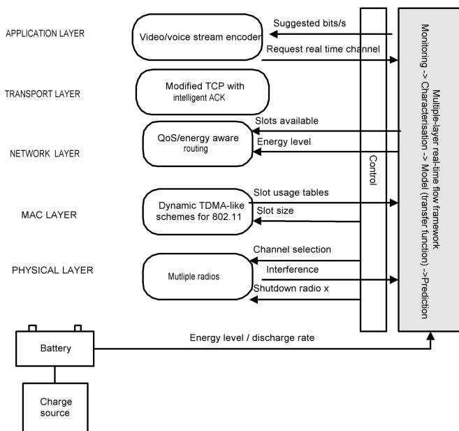
Fig. 3. Real-time flow Framework architecture showing possible messages that can be sent or received from various communication layers
