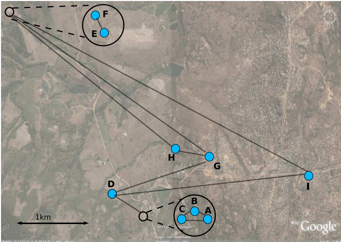
Fig. 1. A map of the Peebles valley mesh. Each solid dot represents a wireless node. An empty dot represents a close cluster of nodes shown in the circles. The area on the left is wealthy farm land and the area on the right is poorer tribal land.
